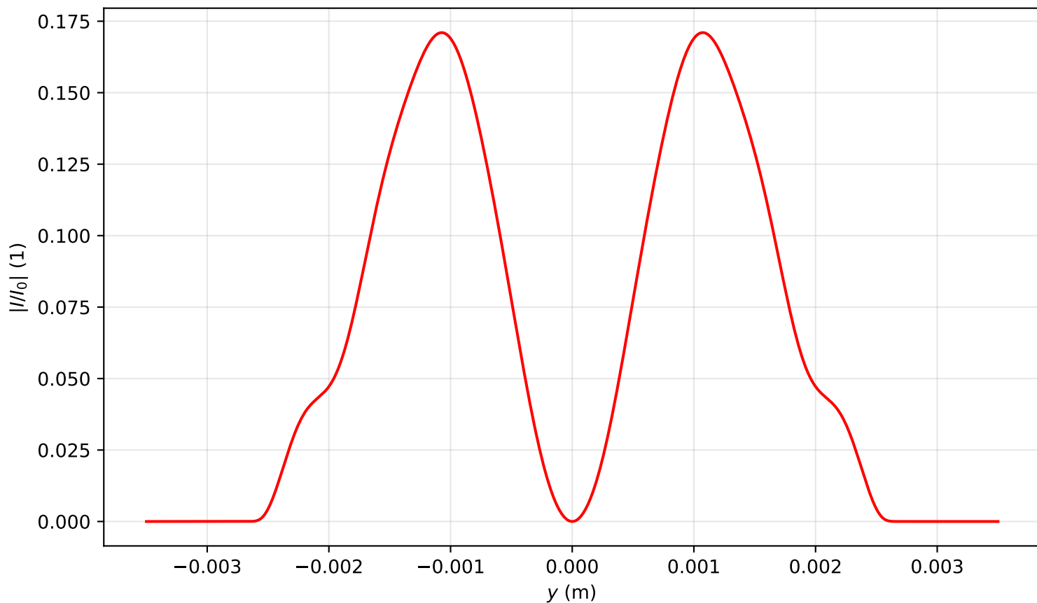
Intensity profile I(x=0, y, z=3.981)/I_0 , \text{Pin}=0.5\text{Pcr} , artificial time
